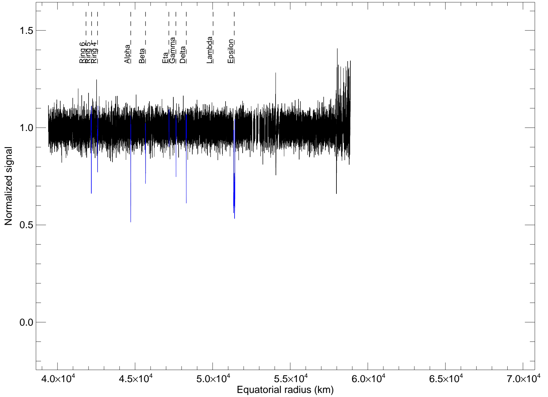
u65_irtf_320cm_2200nm rings egress
