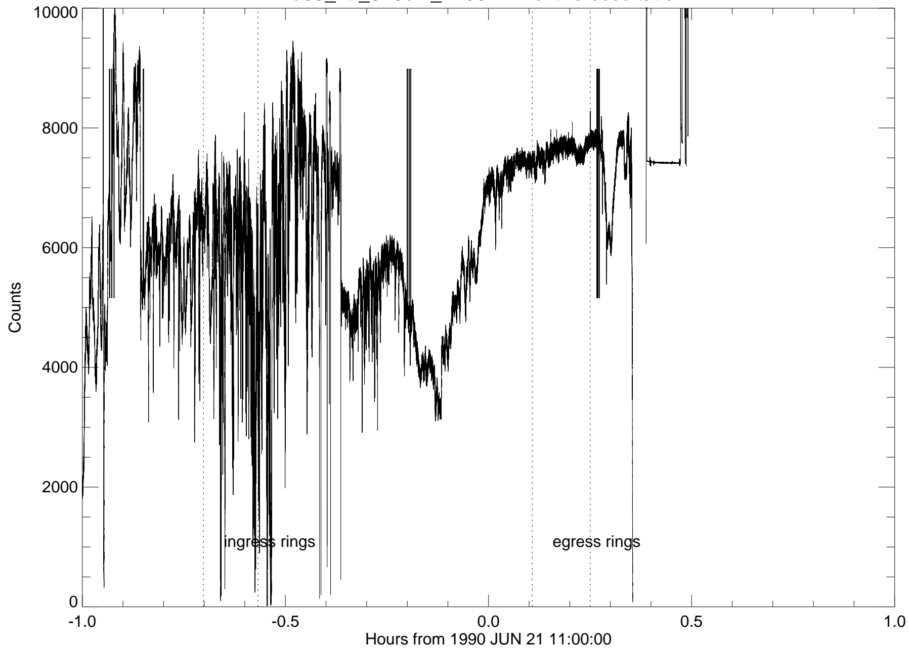
u65_irtf_320cm_2200nm - entire occultation
