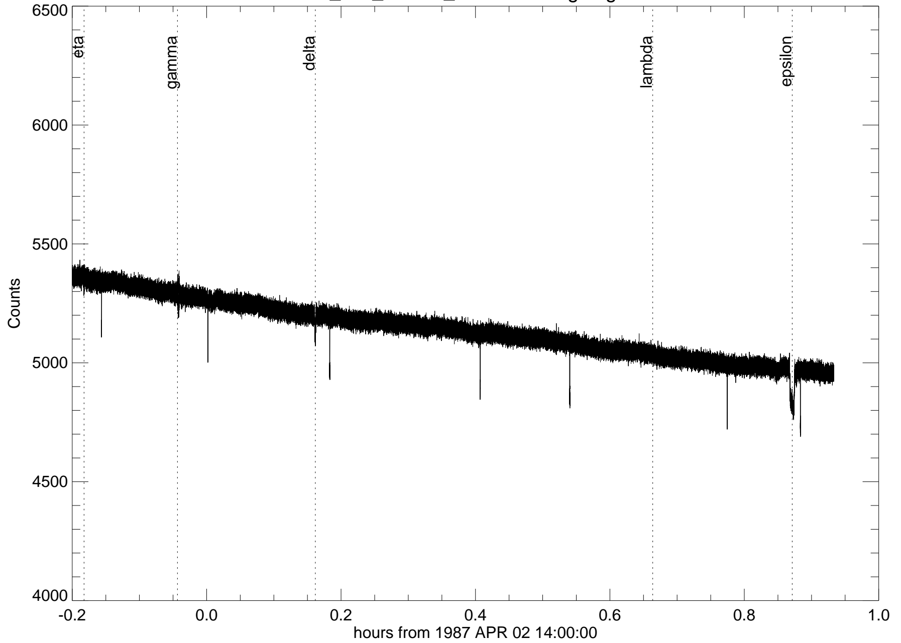
u36_sso_390cm_2200nm - rings egress
