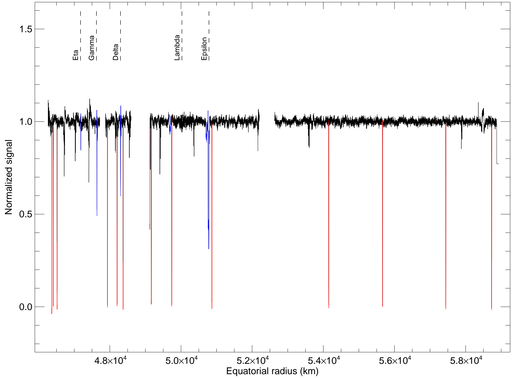
u36_irtf_320cm_2200nm rings egress
