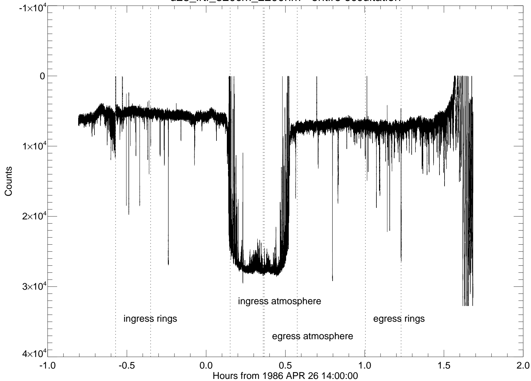
u28_irtf_320cm_2200nm - entire occultation
