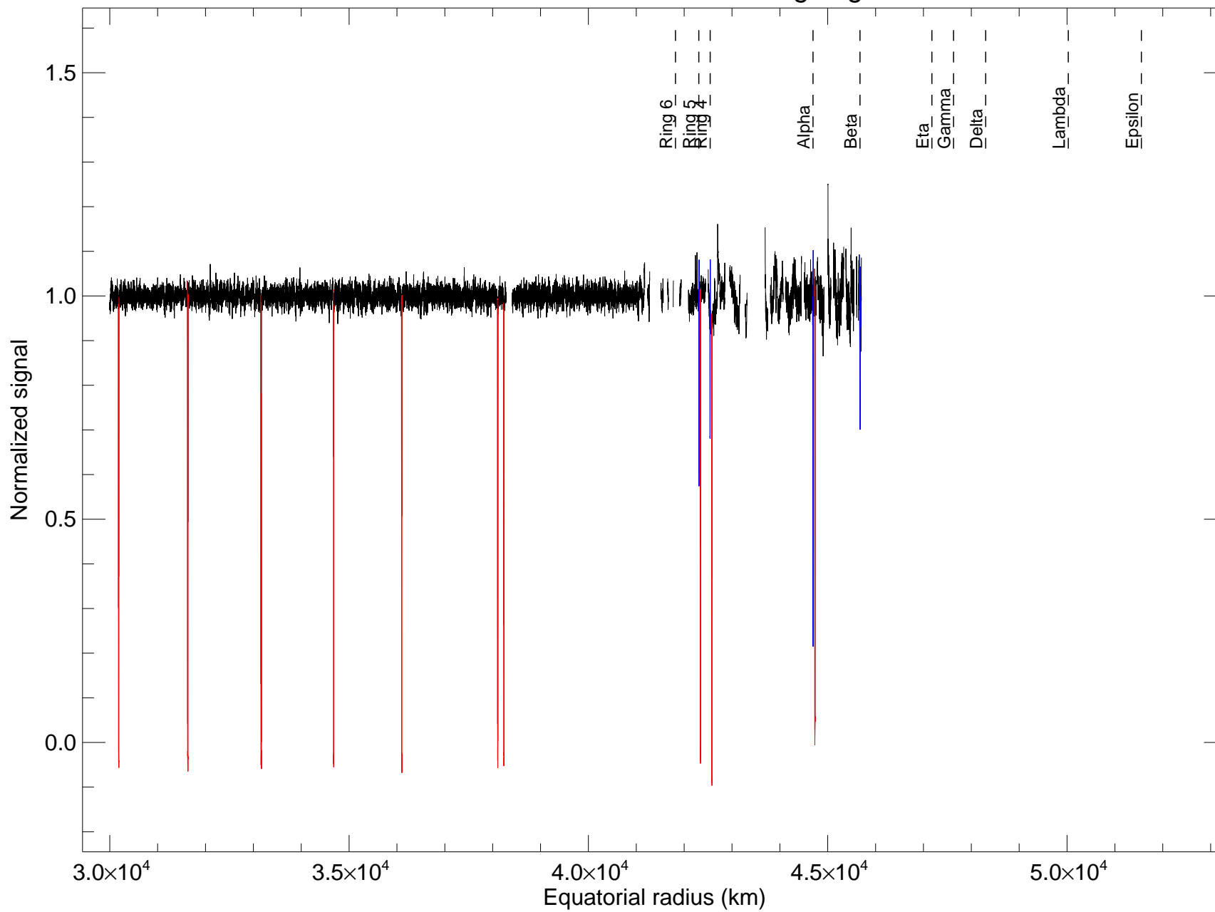
u17b_saao_188cm_2220nm rings egress
