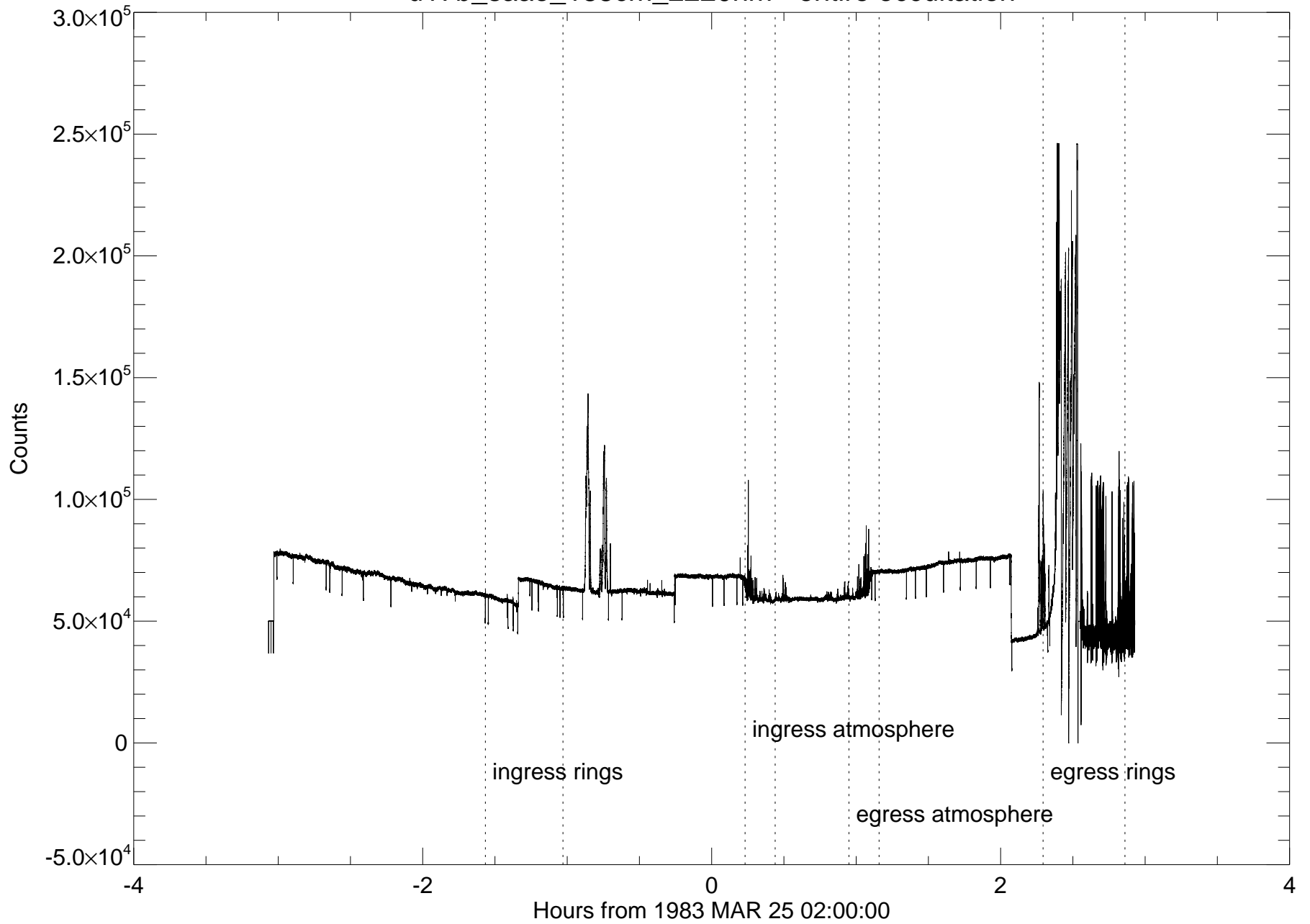
u17b_saao_188cm_2220nm - entire occultation
