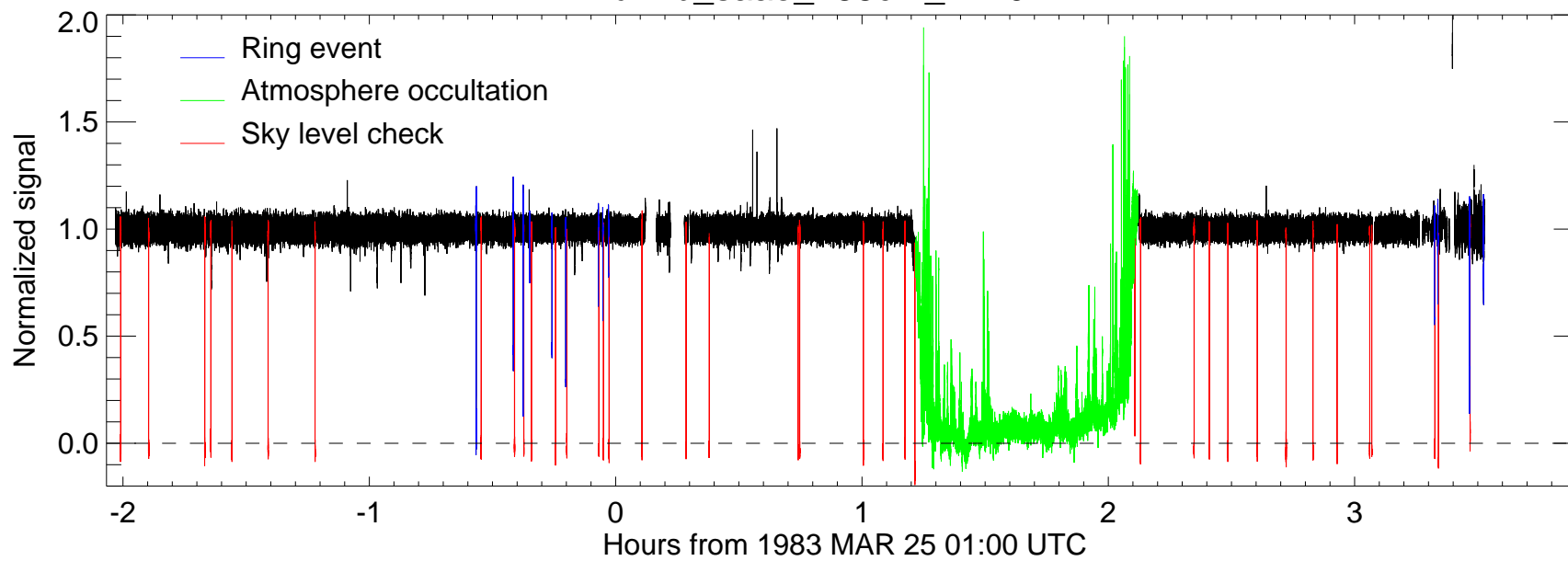
u17b_saao_188cm_2220nm
