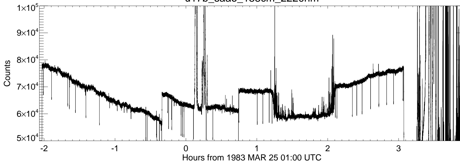
u17b_saao_188cm_2220nm
