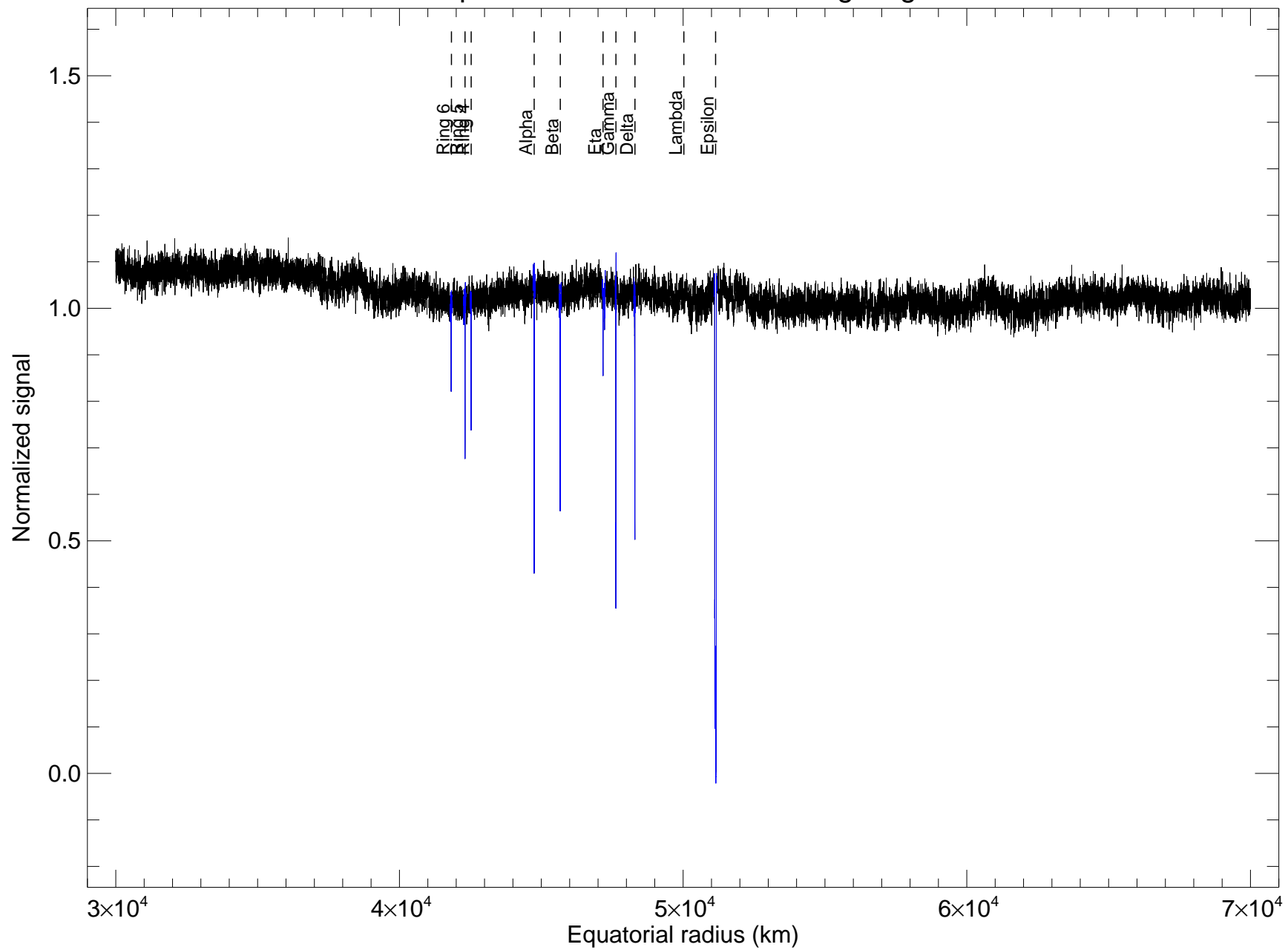
u16_palomar_508cm_2200nm rings ingress
