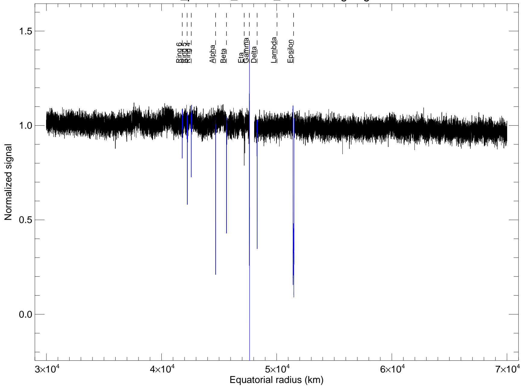
u16_palomar_508cm_2200nm rings egress
