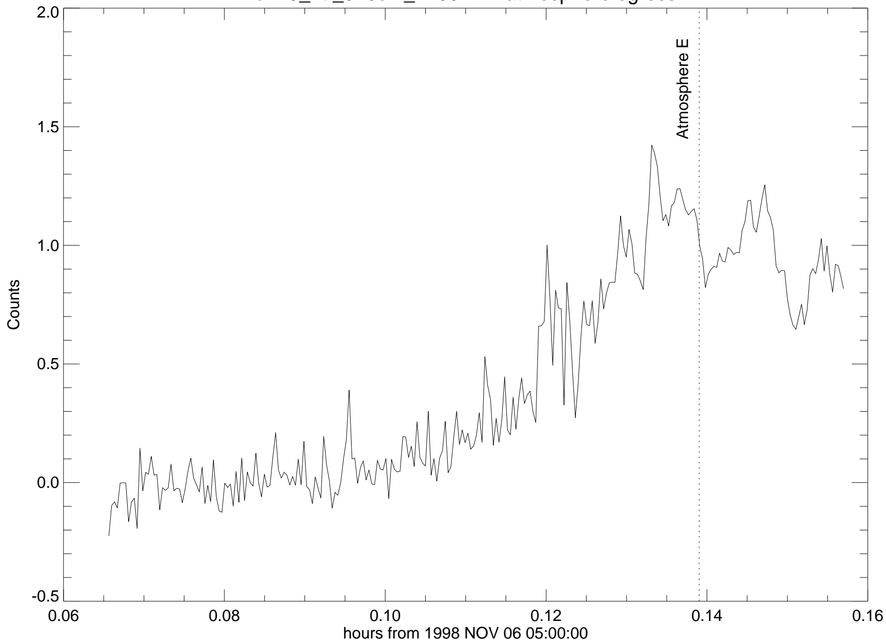
u149_irtf_320cm_2200nm - atmosphere egress
