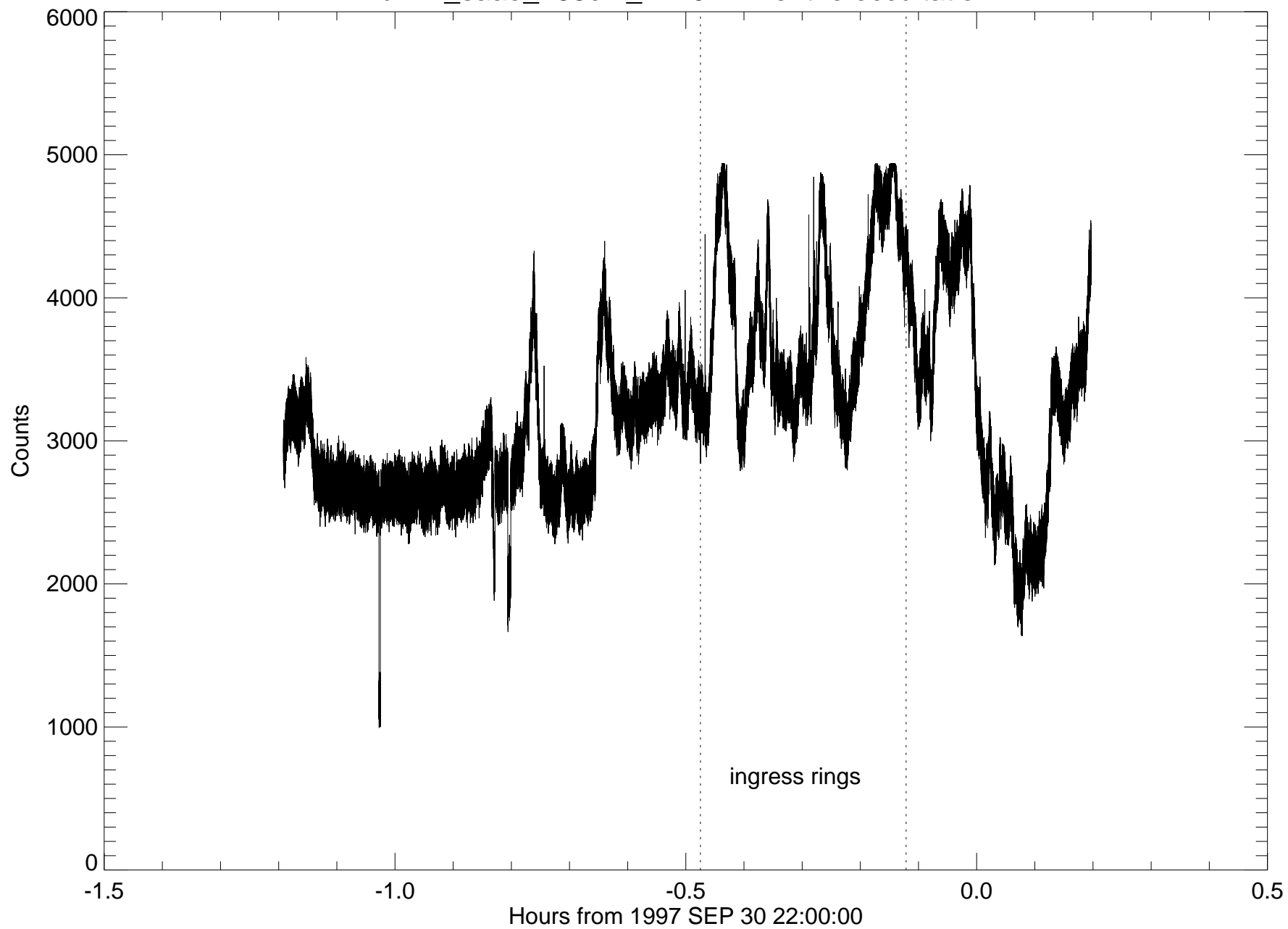
u144_sao_188cm_2220nm - entire occultation
