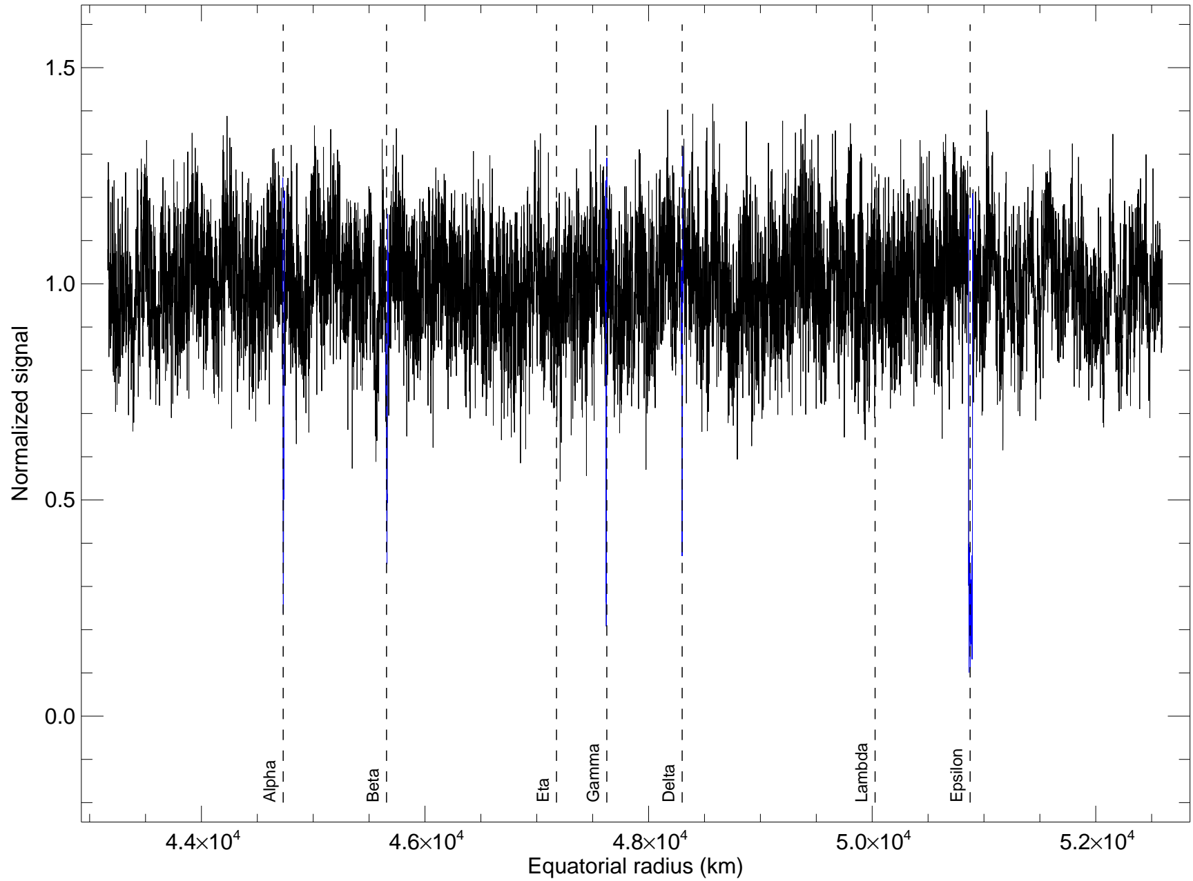
u144_caha_123cm_2200nm rings ingress
