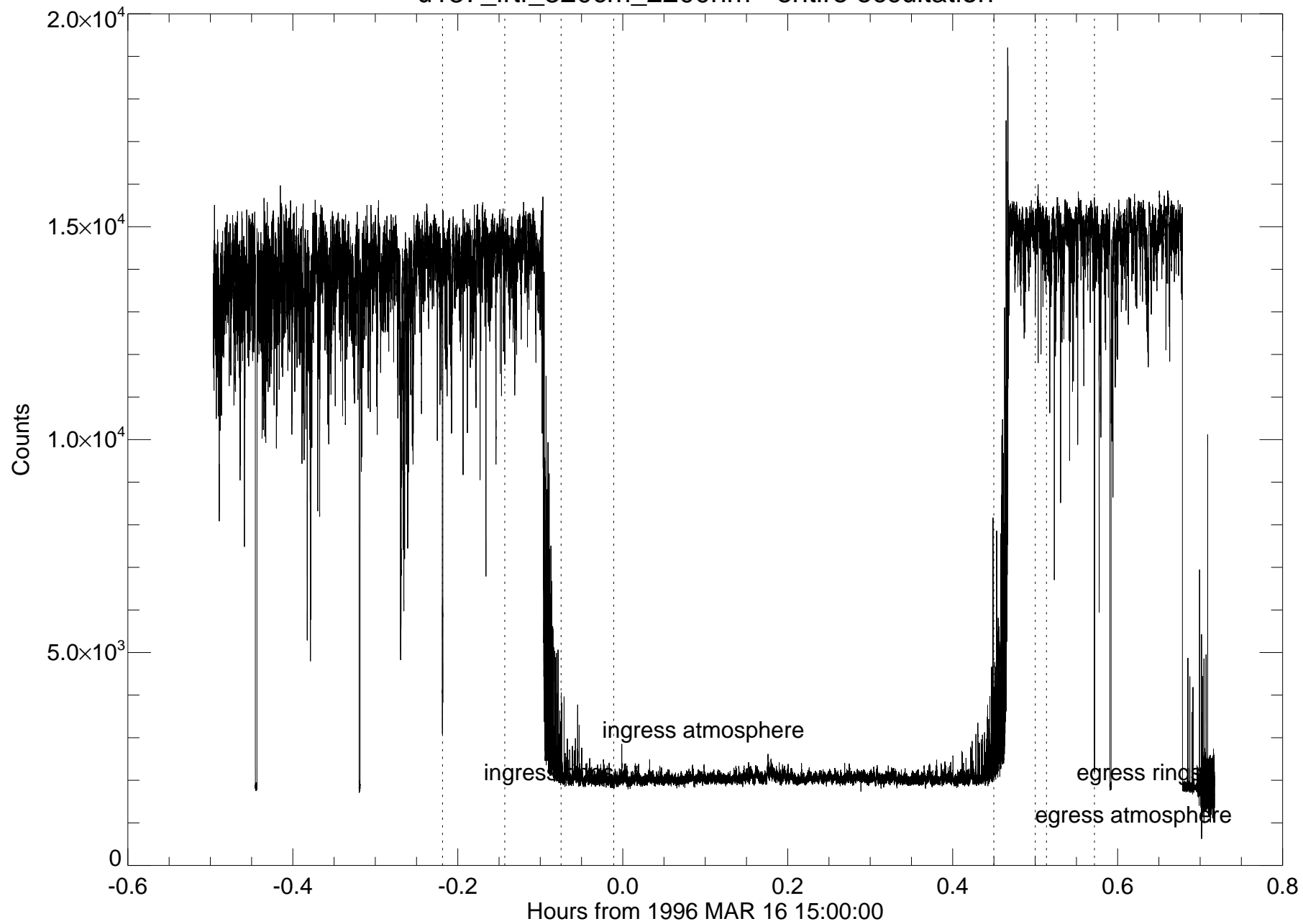
u137_irtf_320cm_2200nm - entire occultation
