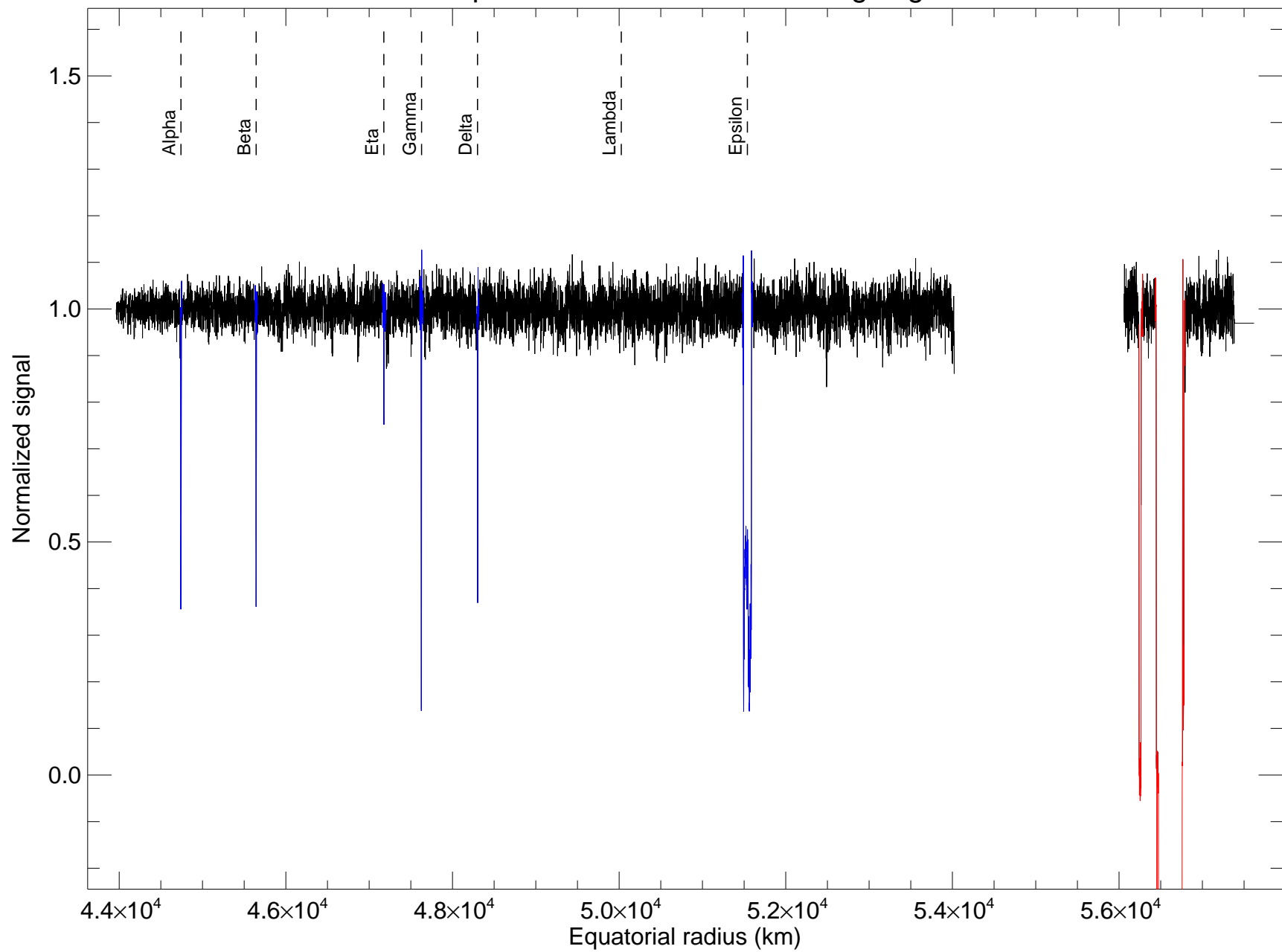
u103_palomar_508cm_2200nm rings egress
