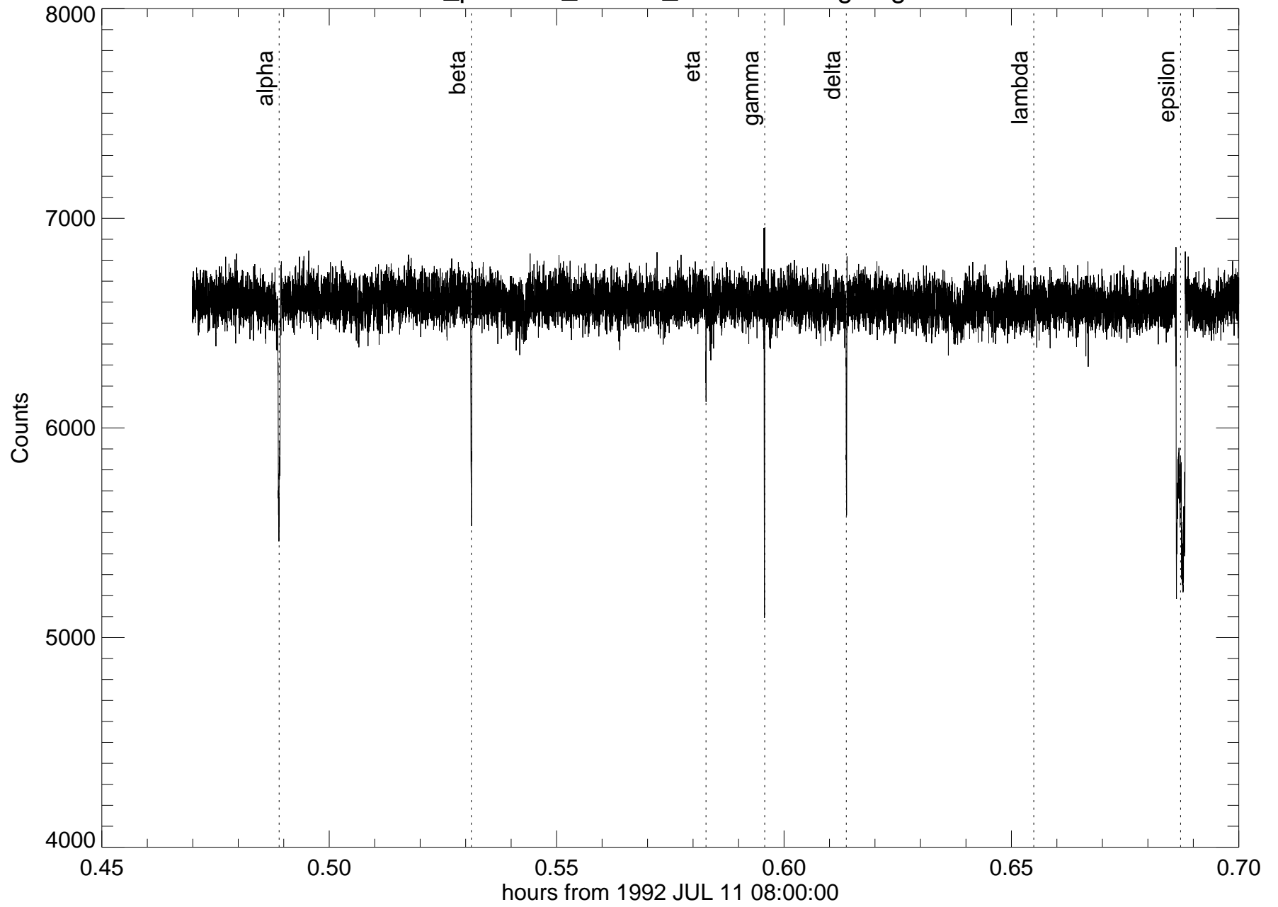
u103_palomar_508cm_2200nm - rings egress
