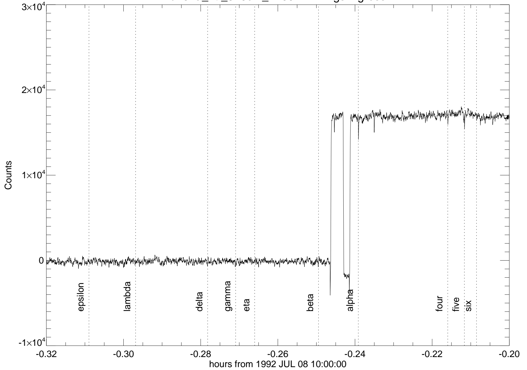
u102a_irtf_320cm_2200nm - rings ingress
