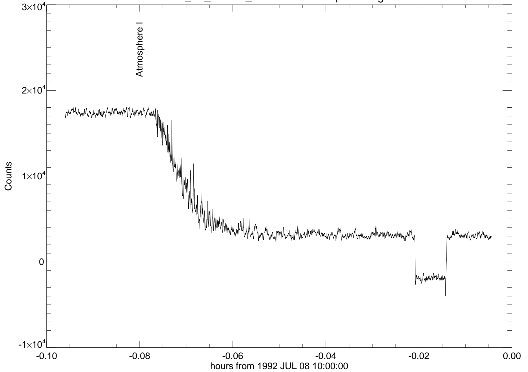
u102a_irtf_320cm_2200nm - atmosphere ingress
