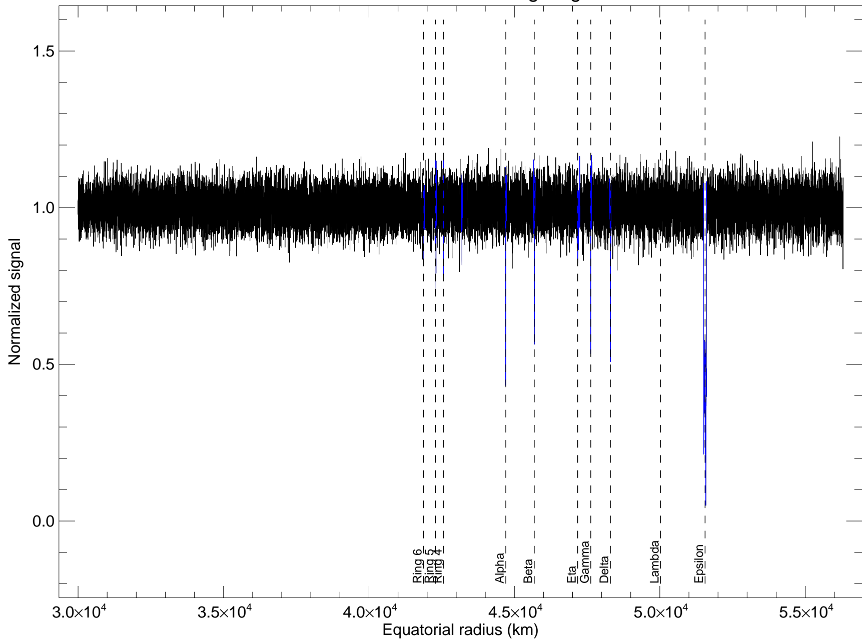
u0_kao_91cm_734nm rings ingress
