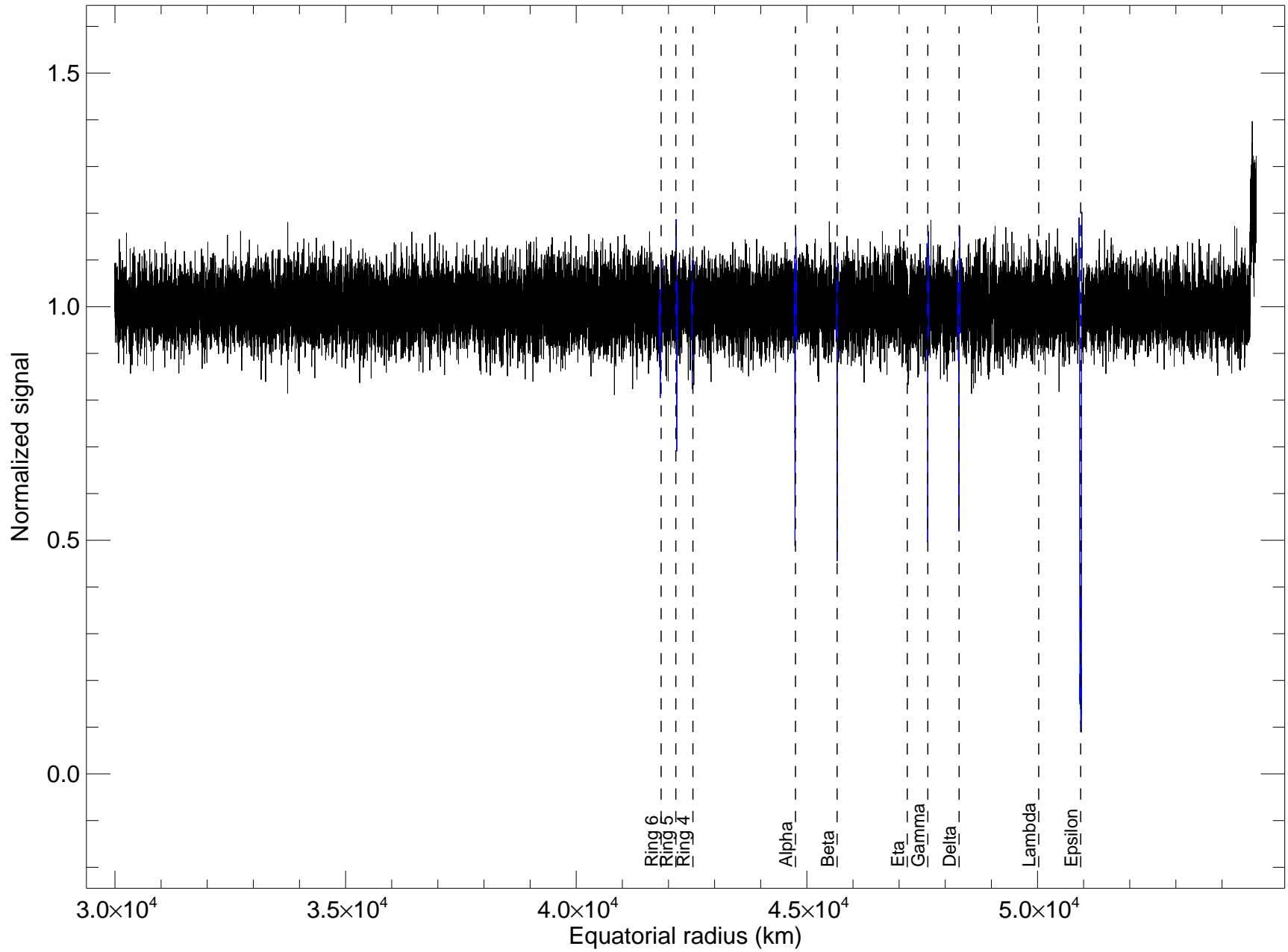
u0_kao_91cm_734nm rings egress
